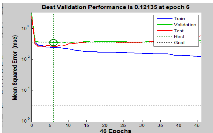
Fig.14. Training- Validation procedure in the proposed LM algorithm.
