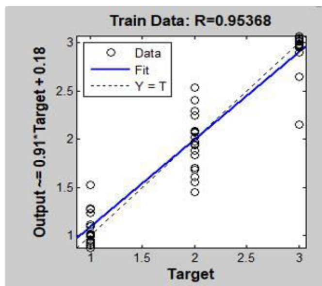
Fig.15. Correlation factor between variables
